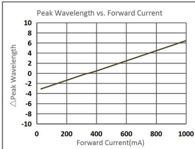
d) Color Shift Characteristics 颜色漂移曲线 ( T_j = 25^\circ\text{C} )
